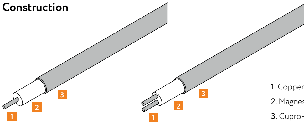
Dual-conductor cable
